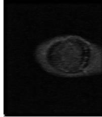
val_images_idx_184/reconstruction
