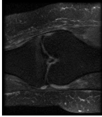
bspline_acc4
