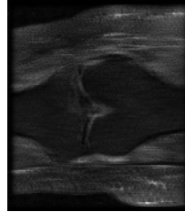
fourier_acc4
