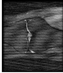
val_images_idx_132/target
