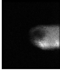
val_images_idx_472/target
