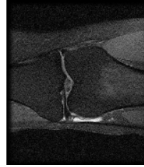
fourier_acc4
