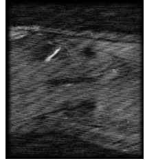
nearest_acc4
