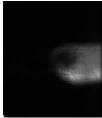
val_images_idx_472/reconstruction
