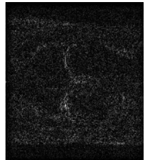
nearest_acc4
