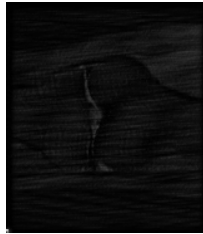
val_images_idx_132/reconstruction
